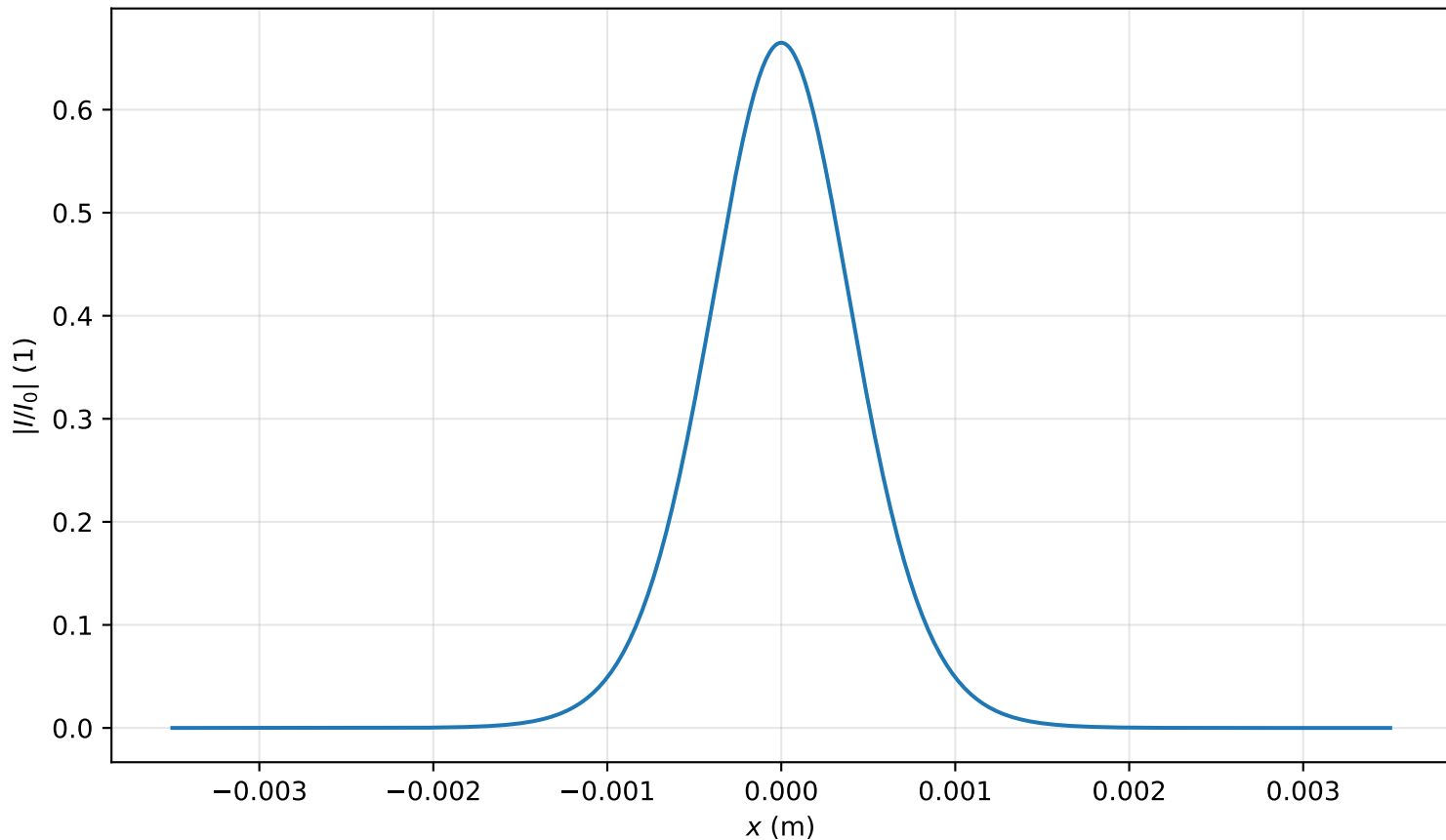
Intensity profile I(x, y = 0, z = 2.229m)/I_0 , P_{in}=0.4P_{cr} , artificial time
